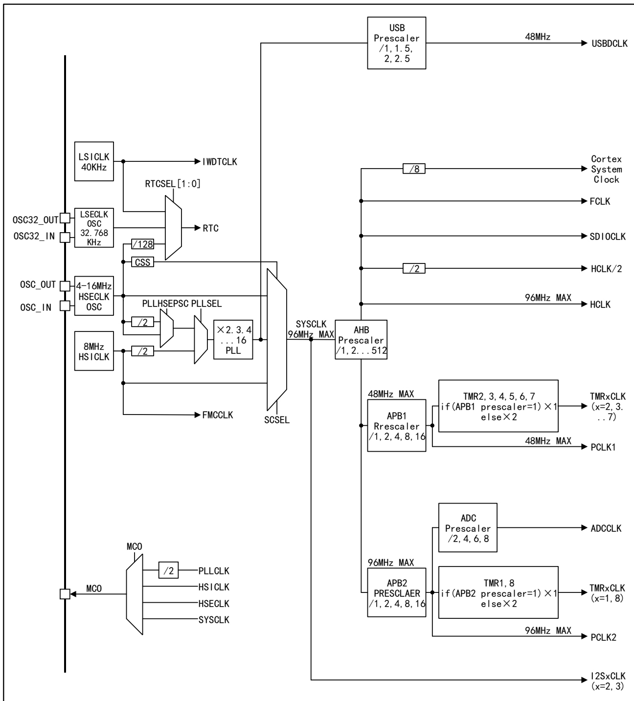
Figure 4 APM32F103RCT7 Clock Tree
